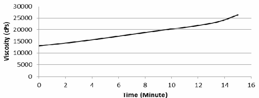
Changes in viscosity with time for GL305 at 25°C
